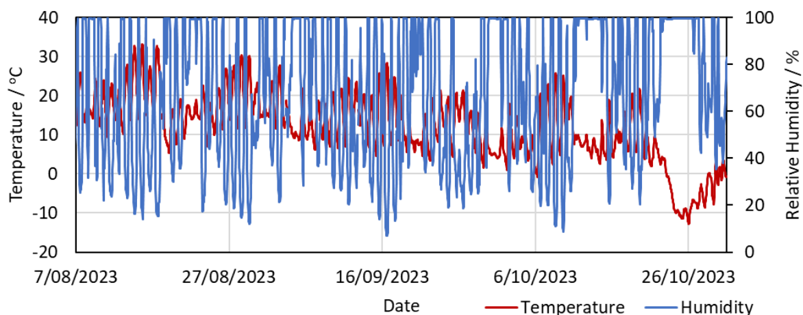
Figure 3: Relative humidity and temperature for the test period.
