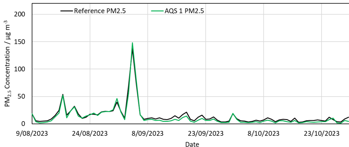
Figure 10: 24-hour time series data showing AQS 1 PM 2.5 data and the Teledyne T640 PM 2.5 data from August 9 th to October 30 th , 2023, for the Calgary Inglewood reference station.
