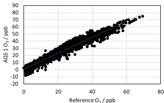
Figure 5: Scatter plot comparing hourly AQS 1 ozone module and Thermo Scientific Ozone Analyzer data for the Calgary Inglewood station from August 9 th to October 30 th , 2023.
