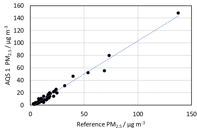
Figure 11: Scatter plot comparing the 24-hour AQS 1 PM 2.5 data and the Teledyne T640 PM 2.5 data from August 9 th to October 30 th , 2023, for the Calgary Inglewood reference station.
