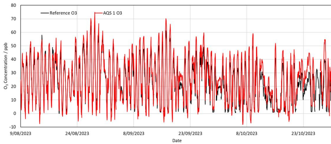
Figure 4: Hourly time series data for AQS 1 and Thermo Scientific Ozone Analyzer from August 9 th to October 30 th , 2023, for the Calgary Inglewood station.
