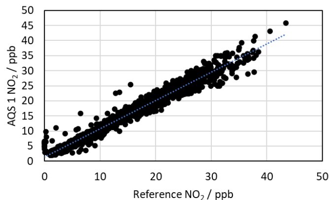
Figure 8: Scatter plot comparing hourly AQS 1 NO 2 module and Thermo Scientific NO-NO 2 -NO x Analyzer data for the Calgary Inglewood station from August 9 th to October 30 th , 2023.
