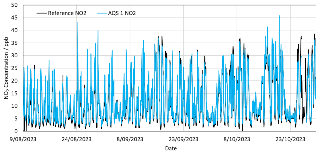
Figure 7: Hourly time series for AQS 1 and Thermo Scientific NO-NO 2 -NO x Analyzer from August 9 th to October 30 th , 2023, for the Calgary Inglewood station.
